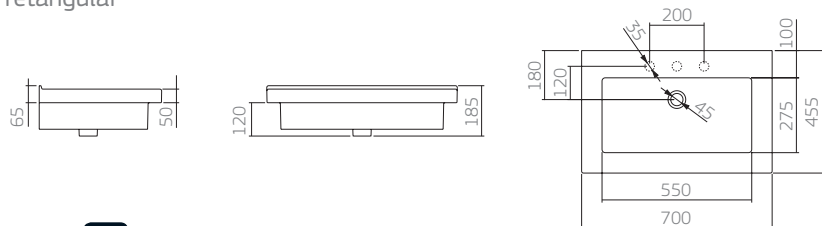
L.94 cuba retangular
