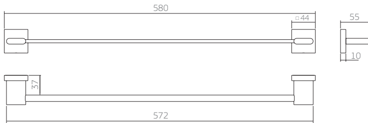
2040.C33.050 porta-toalha barra
