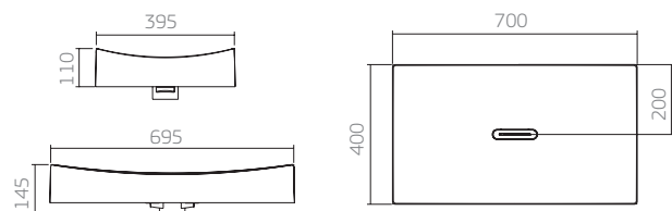
L.1055 cuba retangular
